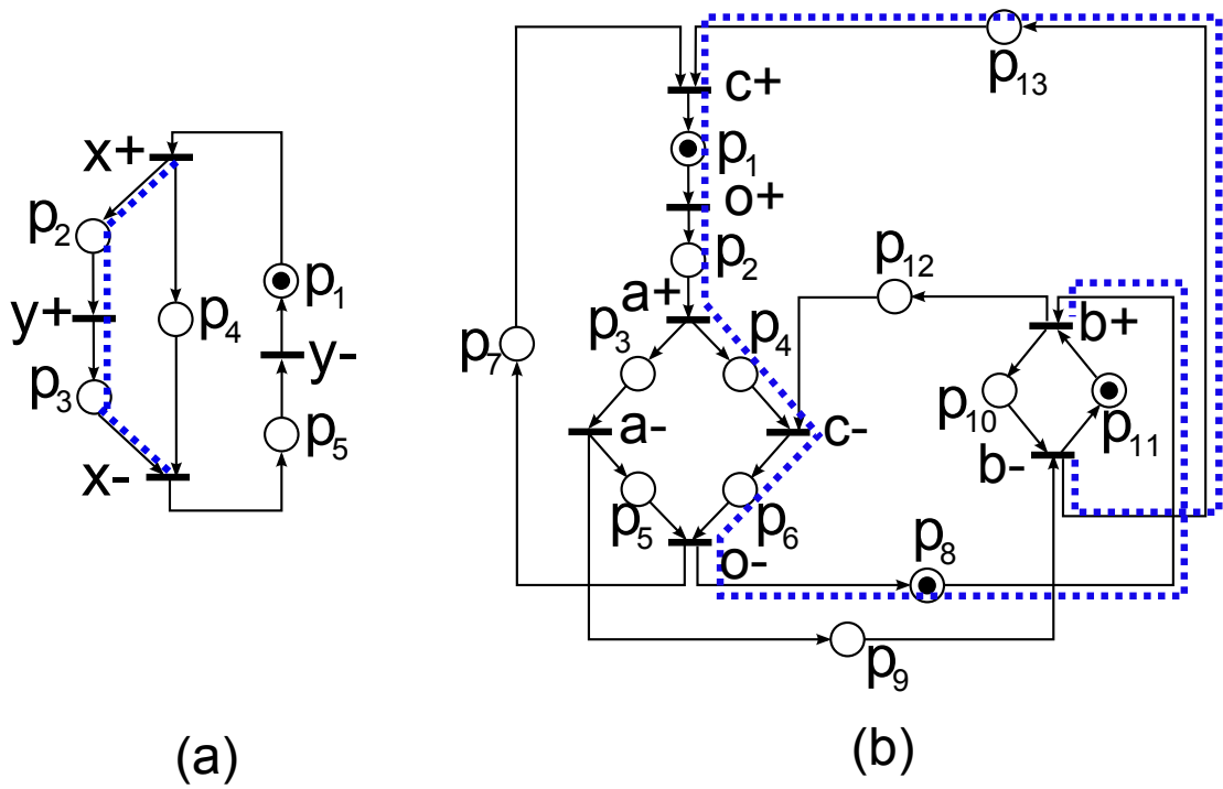
Figure 5.14: Property of shortcut places -
