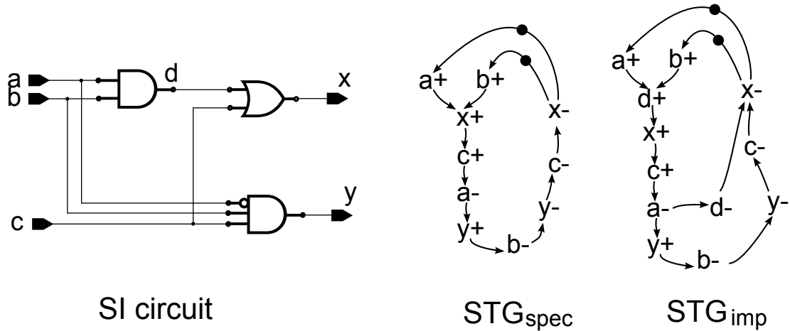
Figure 3.3: An SI circuit with its STG_{spec} and STG_{imp} -
