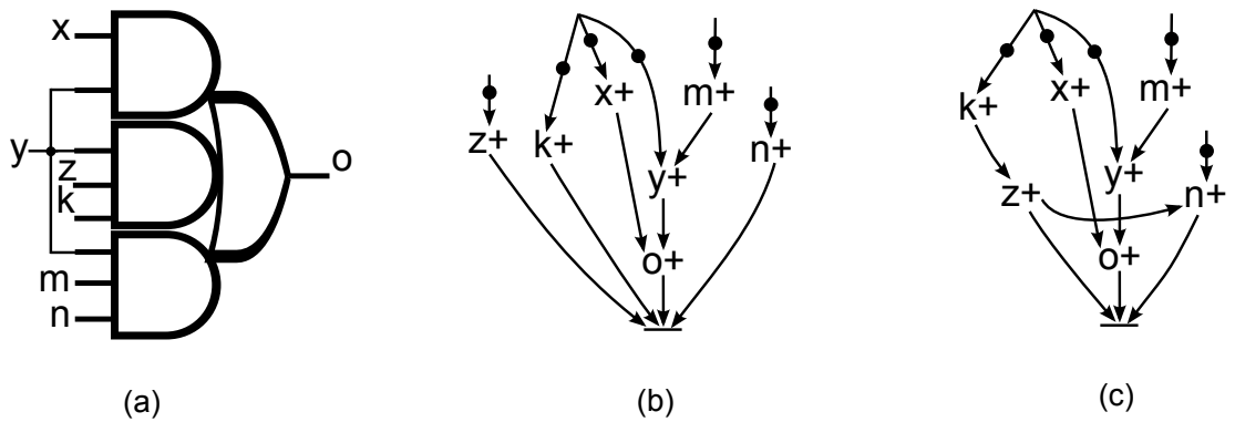
Figure 6.2: Candidate clause and transition for OR-causality in relaxation case 2. (a) the gate, (b) and (c) two different STG segments -
