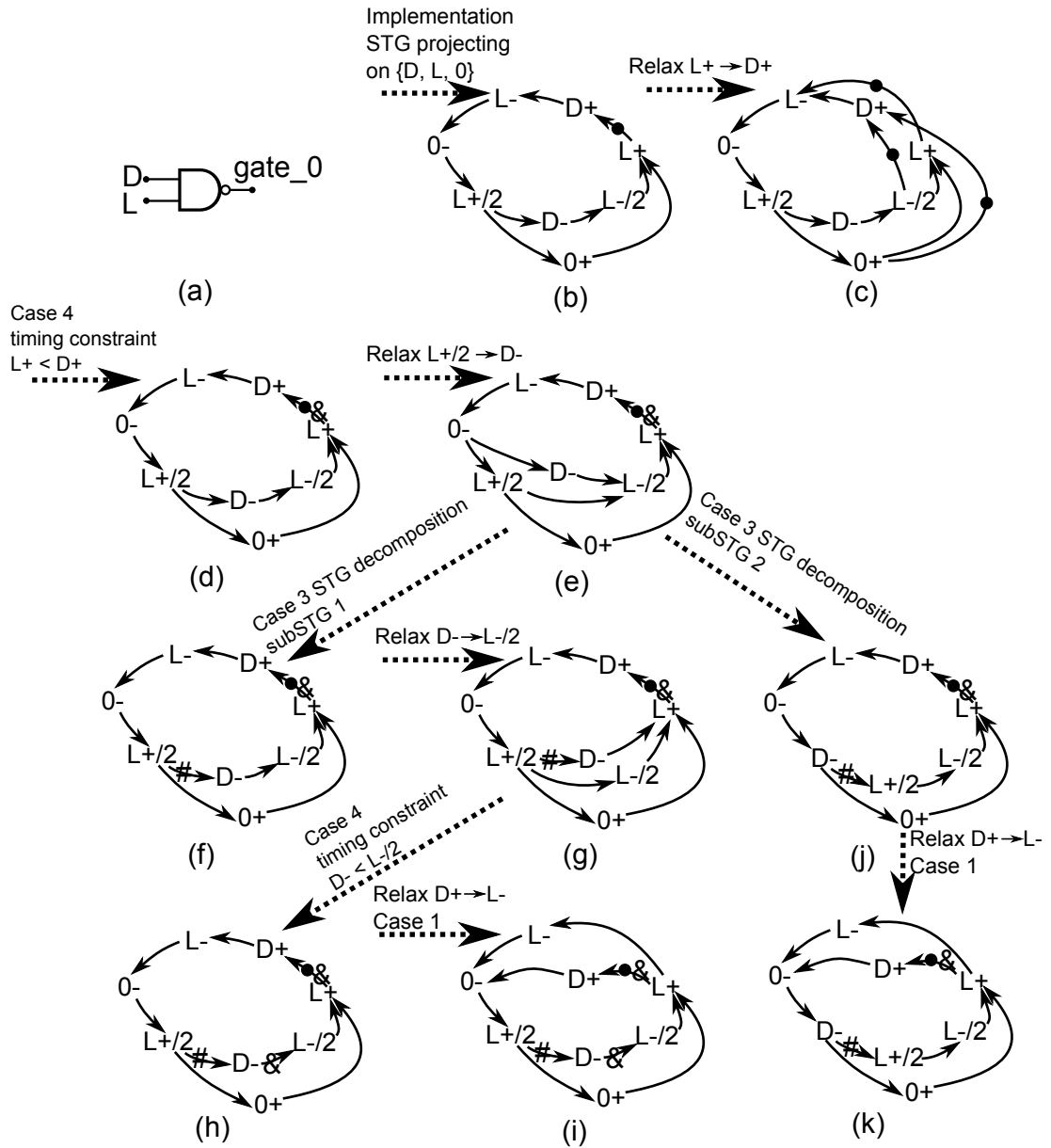
Figure 7.3: The STG relaxation procedure of the gate_0 -
