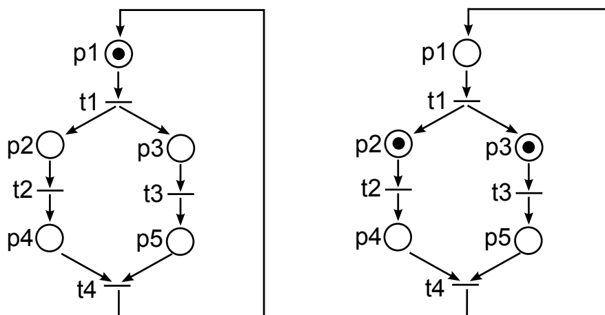
Figure 3.1: A PN example -
