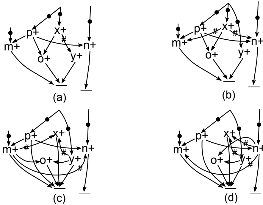
Figure 6.9: Decomposition results for the OR-causality relation in Figure 6.8. (a)-(d) resulting subSTG segments -
