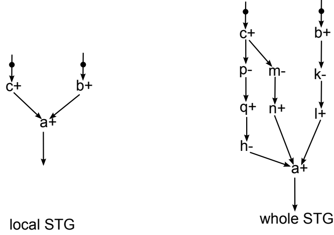
Figure 5.24: Calculate the weight of an arc from STG_{imp} -
