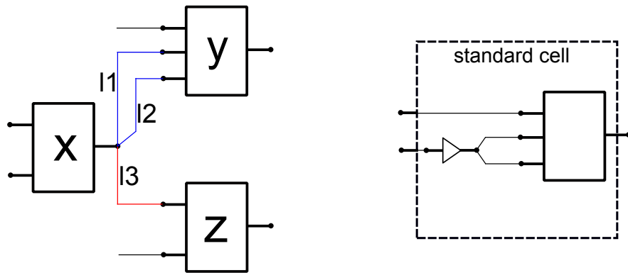
Figure 4.5: Intra operator fork timing assumption -
