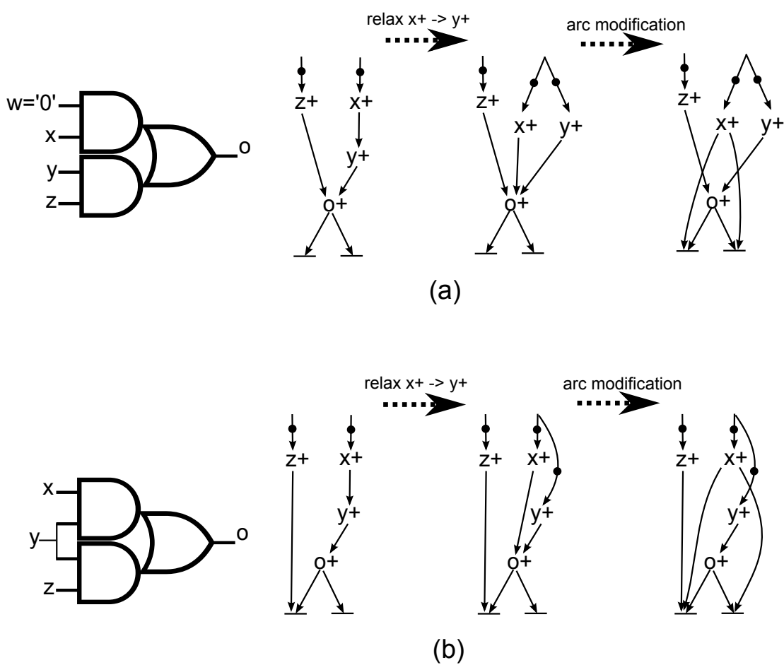
Figure 5.21: Arc modification in case 2. (a) without OR-causality and (b) with OR-causality. -
