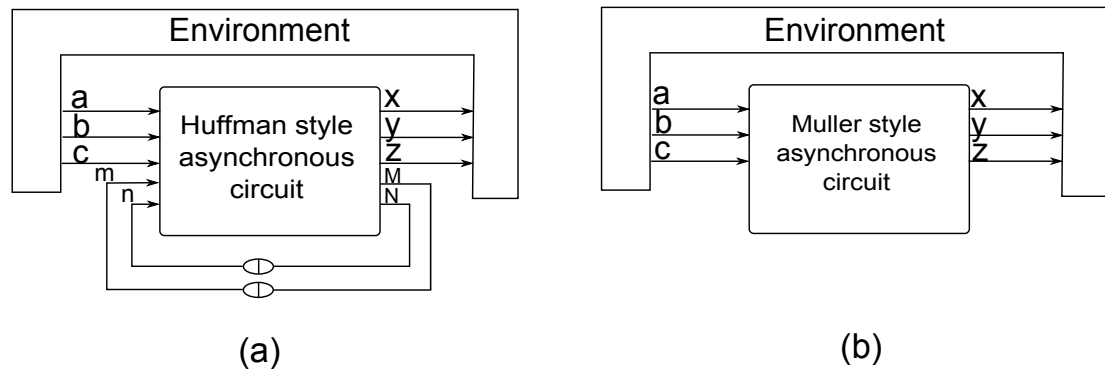
Figure 2.3: The Huffman style asynchronous circuit and the Muller style asynchronous circuit -
