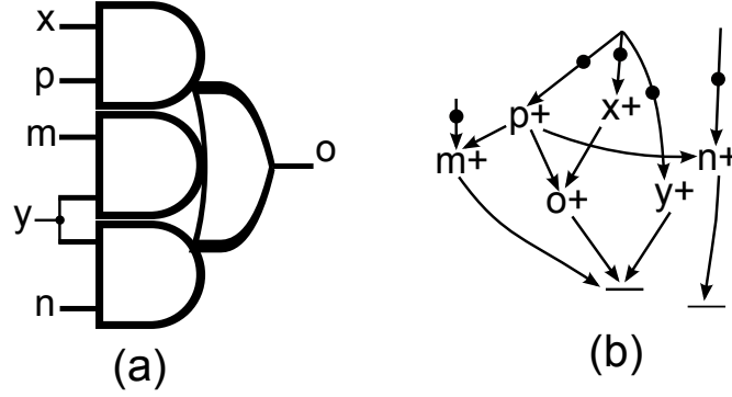
Figure 6.8: An OR-causality relation in case 3. (a) the gate and (b) its local STG segment -
