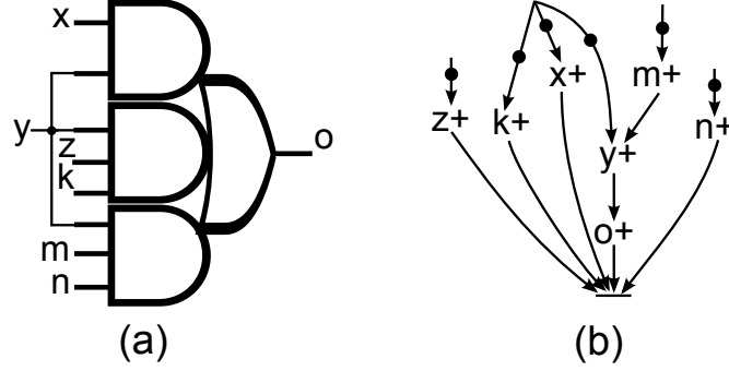
Figure 6.6: An OR-causality relation in case 2. (a) the gate and (b) its local STG segment -
