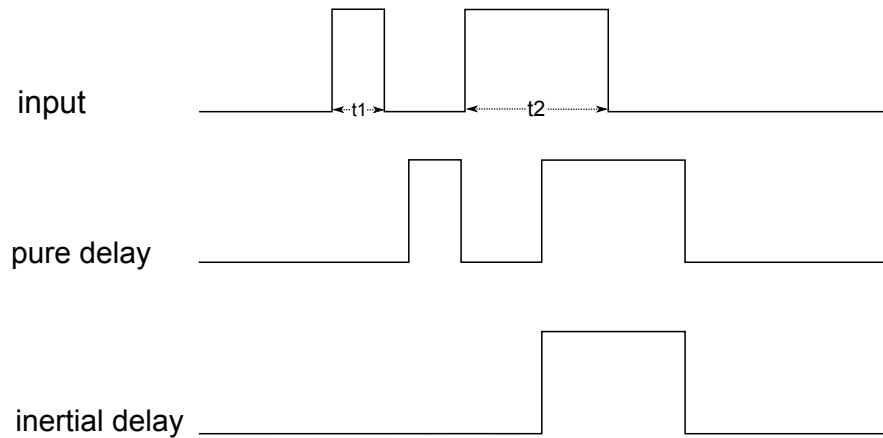
Figure 2.2: Pure delay and inertial delay -
