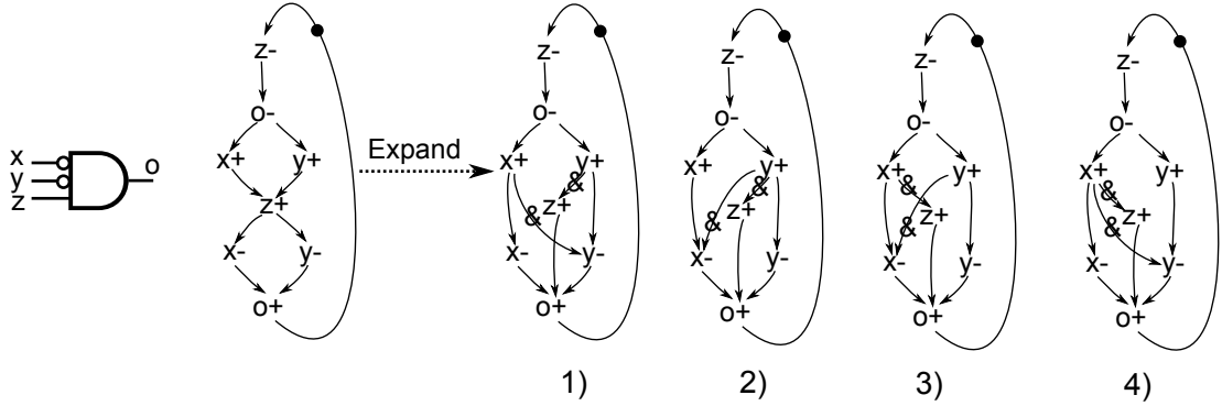
Figure 5.23: Different timing constraints due to different relaxation ordering -
