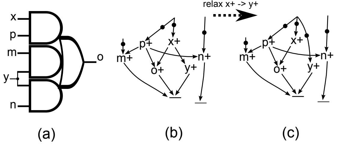
Figure 6.3: OR-causality in relaxation case 3. (a) the gate, (b) and (c) two different STG segments -
