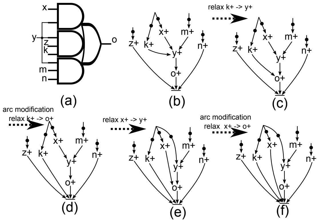
Figure 6.1: OR-causality in relaxation case 2. (a) the gate and (b)-(f) relaxation steps -
