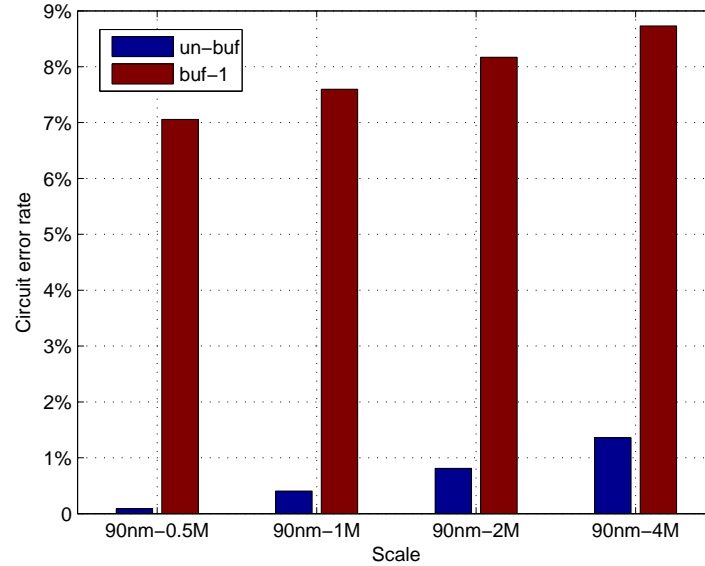
Figure 7.6: The trend of error rate as the scale increases -
