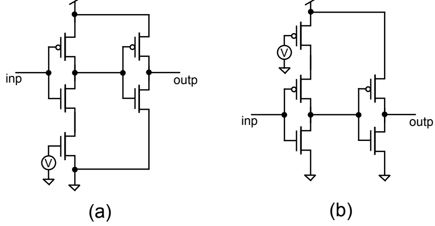
Figure 7.4: The current starved delays. (a) controlled delay for rising transition and (b) controlled delay for falling transition -
