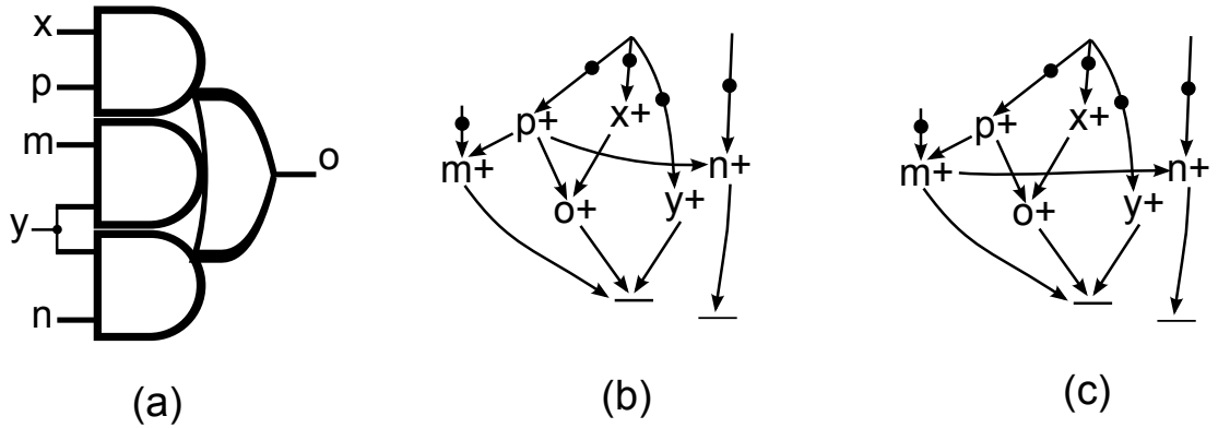
Figure 6.4: Candidate clause and transition for OR-causality in relaxation case 3. (a) the gate, (b) and (c) two different STG segments -
