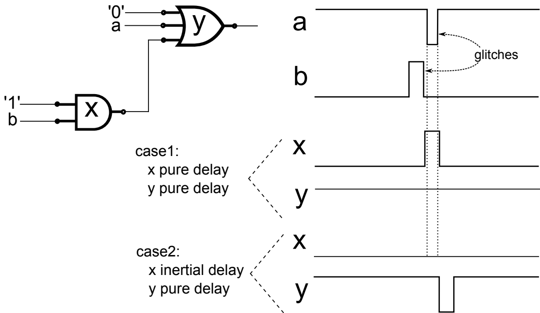
Figure 2.5: Glitches with respect to delay models -
