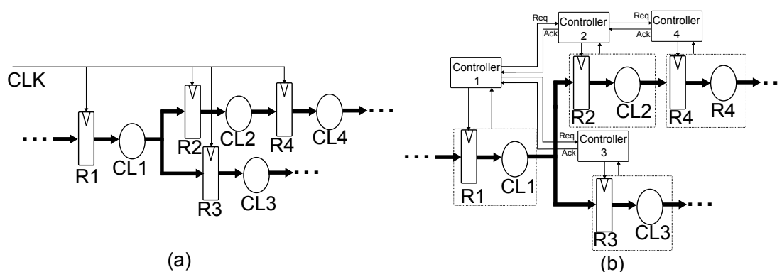
Figure 1.1: A synchronous circuit and the equivalent asynchronous circuit -
