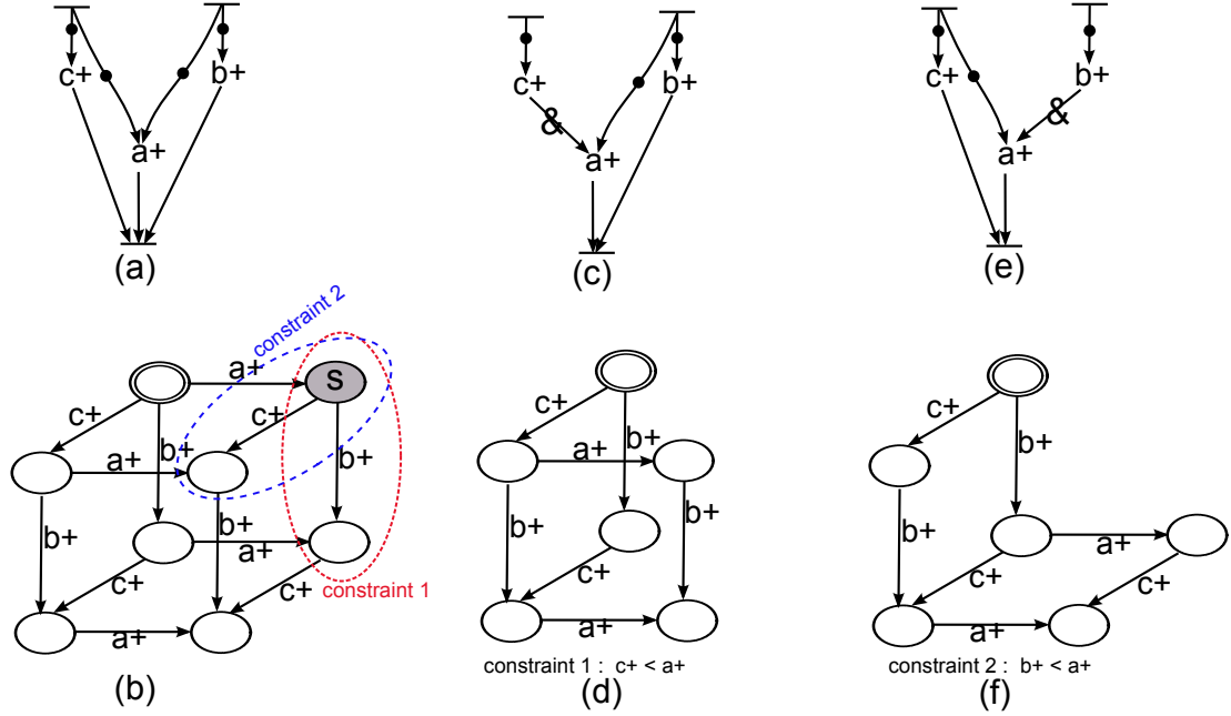
Figure 5.22: Preventing the gate entering hazardous state s -
