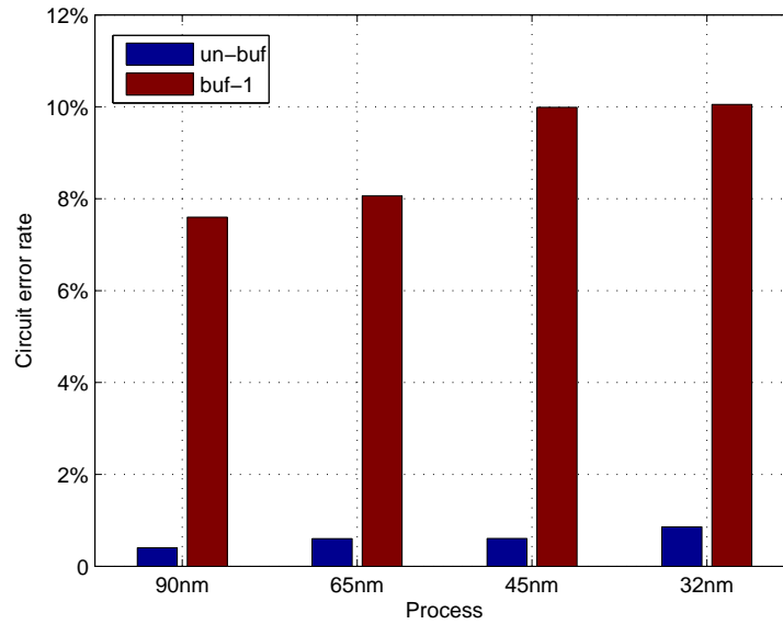
Figure 7.5: The trend of error rate as the technology shrinks -
