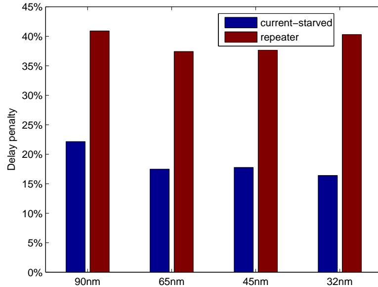
Figure 7.7: The delay penalty -
