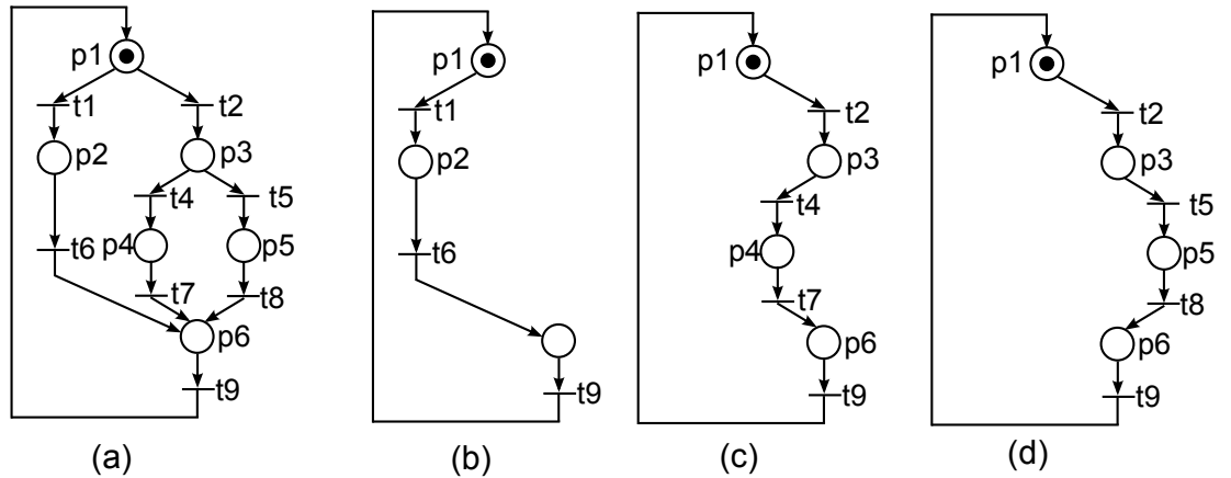
Figure 5.2: A live and safe free-choice PN (a), and its MG components (b)-(d) -
