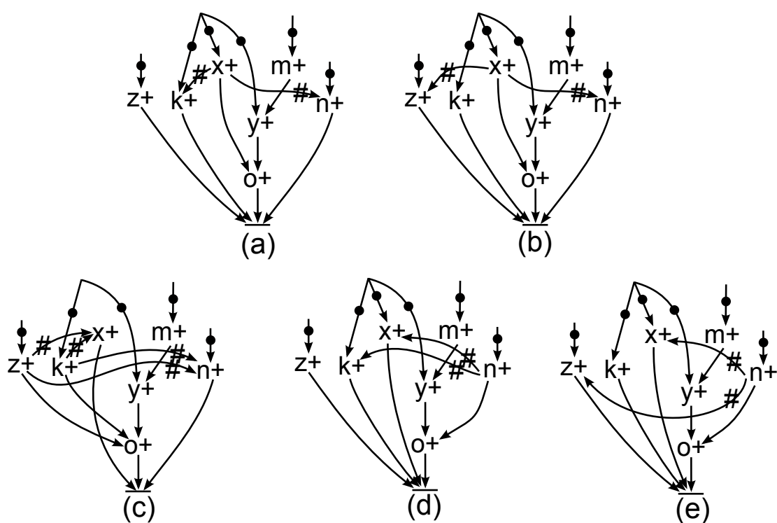
Figure 6.7: Decomposition results for the OR-causality relation in Figure 6.6. (a)-(e) resulting subSTG segments -
