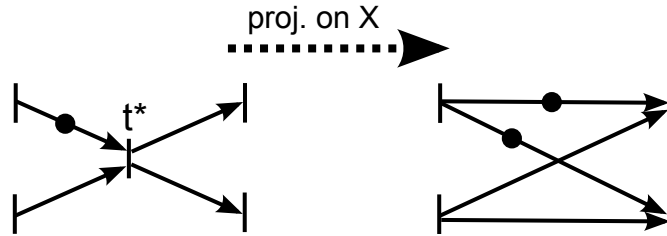
Figure 5.3: Projection of an STG segment on X and t \notin X -
