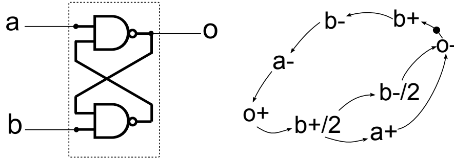
Figure 5.4: An \overline{SR} -latch with its local STG -
