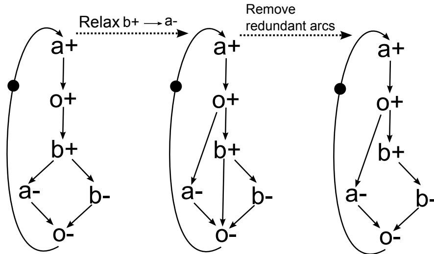
Figure 5.13: redundant arcs due to the relaxation -
