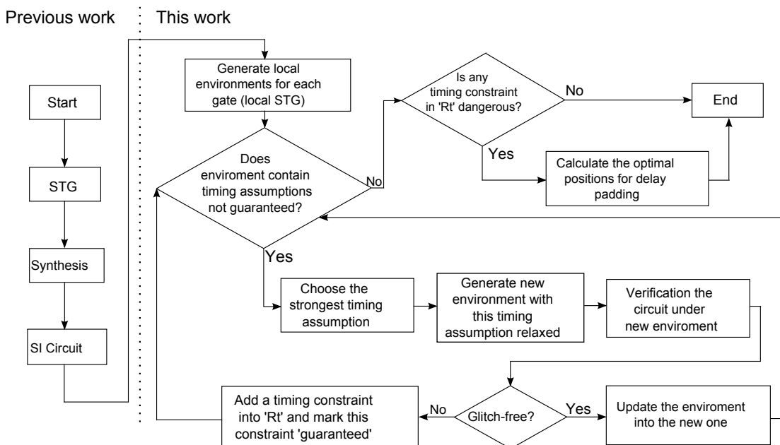
Figure 5.1: The entire flow of this work -
