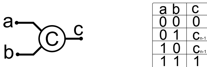
Figure 2.4: A 2-input C-element -
