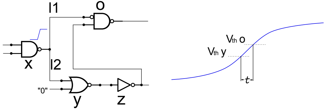
Figure 4.2: Glitch caused by threshold variation -
