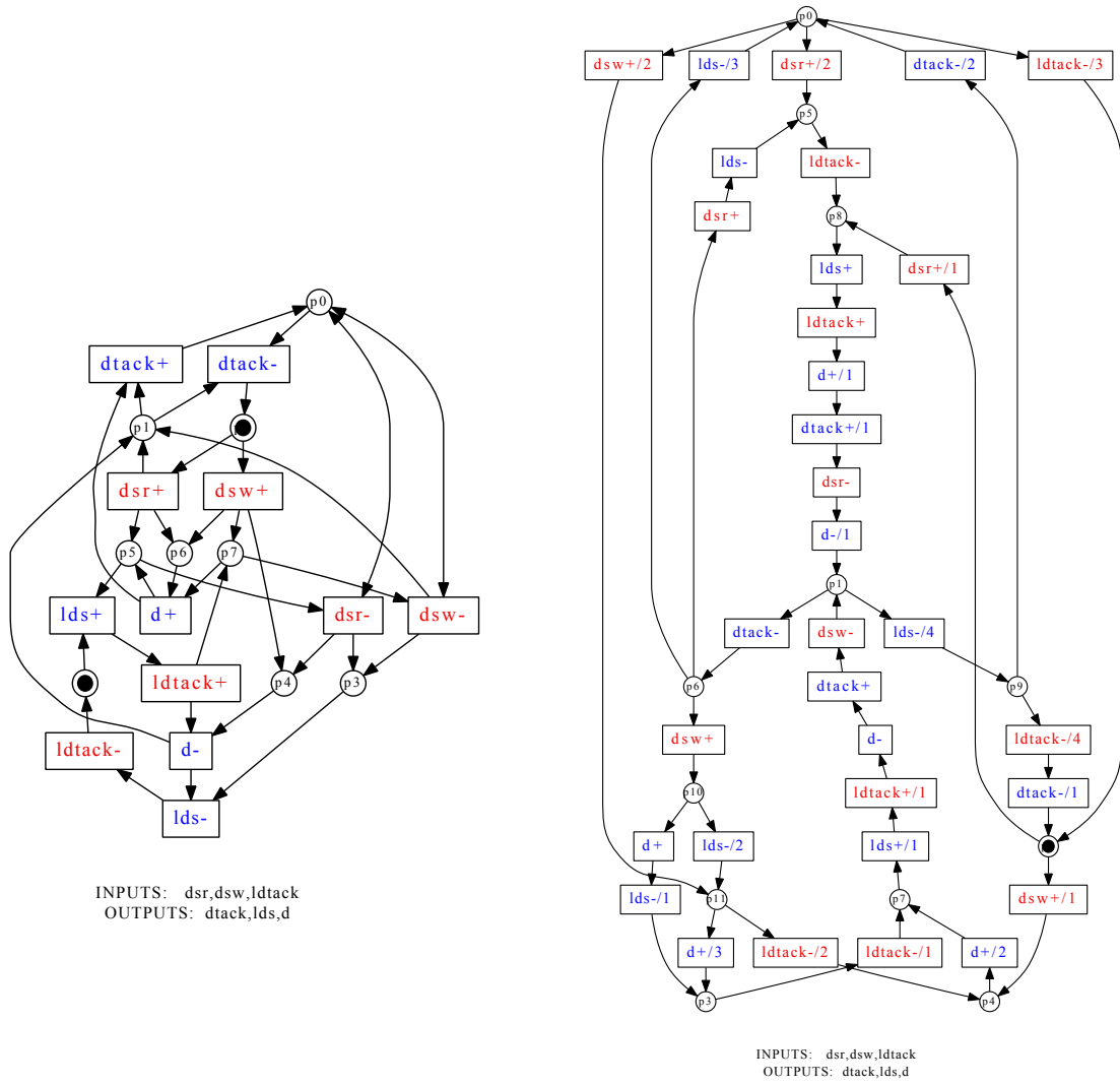
Figure 8.1: A non-free choice STG and its equivalent free-choice STG -
