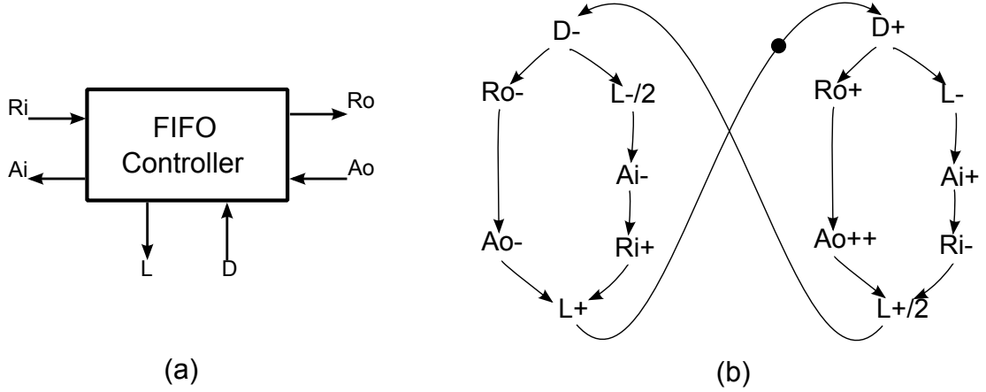
Figure 7.1: The block diagram and STG specification of FIFO -
