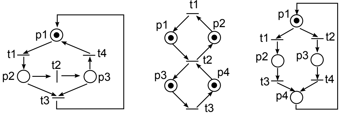
Figure 3.2: PN properties -
