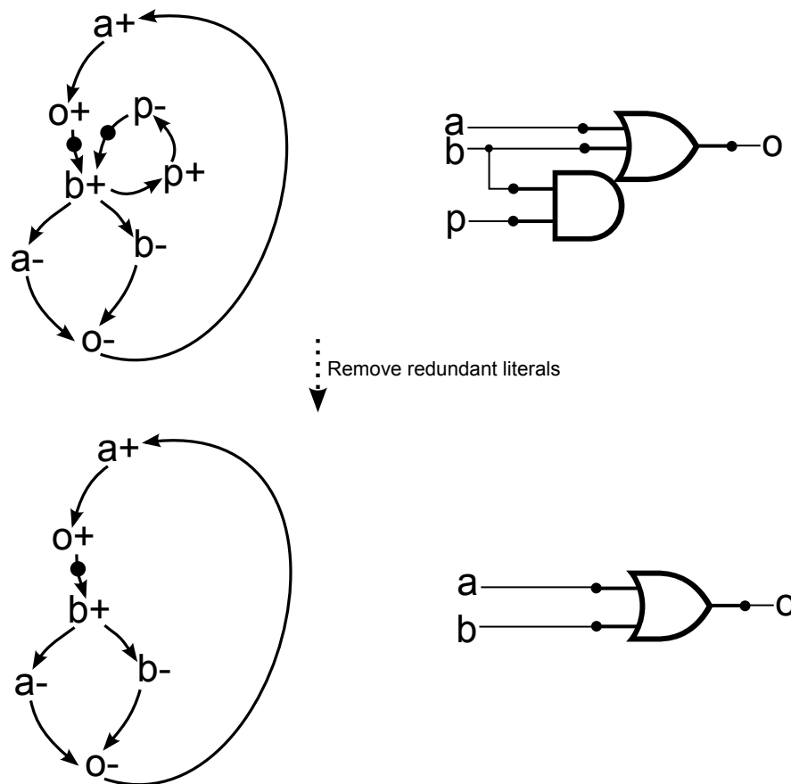
Figure 5.12: Gate o has a redundant literal p -
