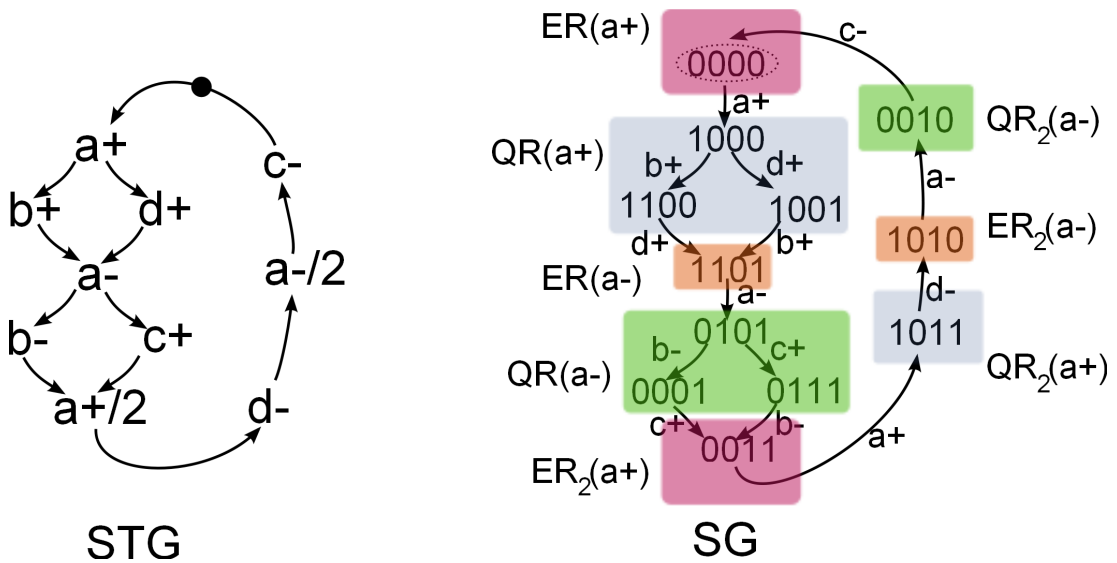
Figure 3.4: An STG with its SG -
