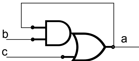
Figure 2.1: A logic gate -
