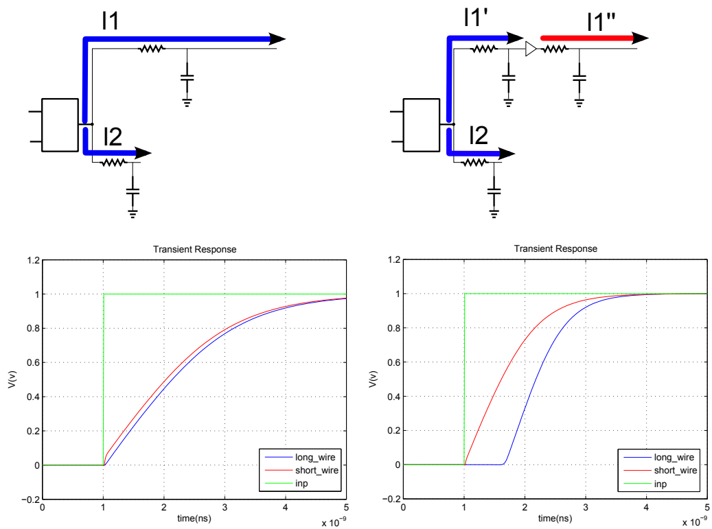
Figure 4.3: Timing difference caused by buffer insertion -
