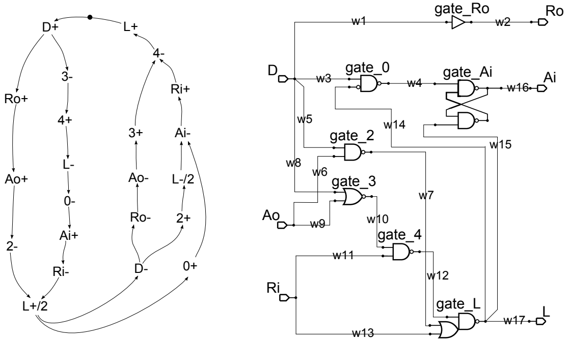
Figure 7.2: The implementation STG and circuit diagram of FIFO -
