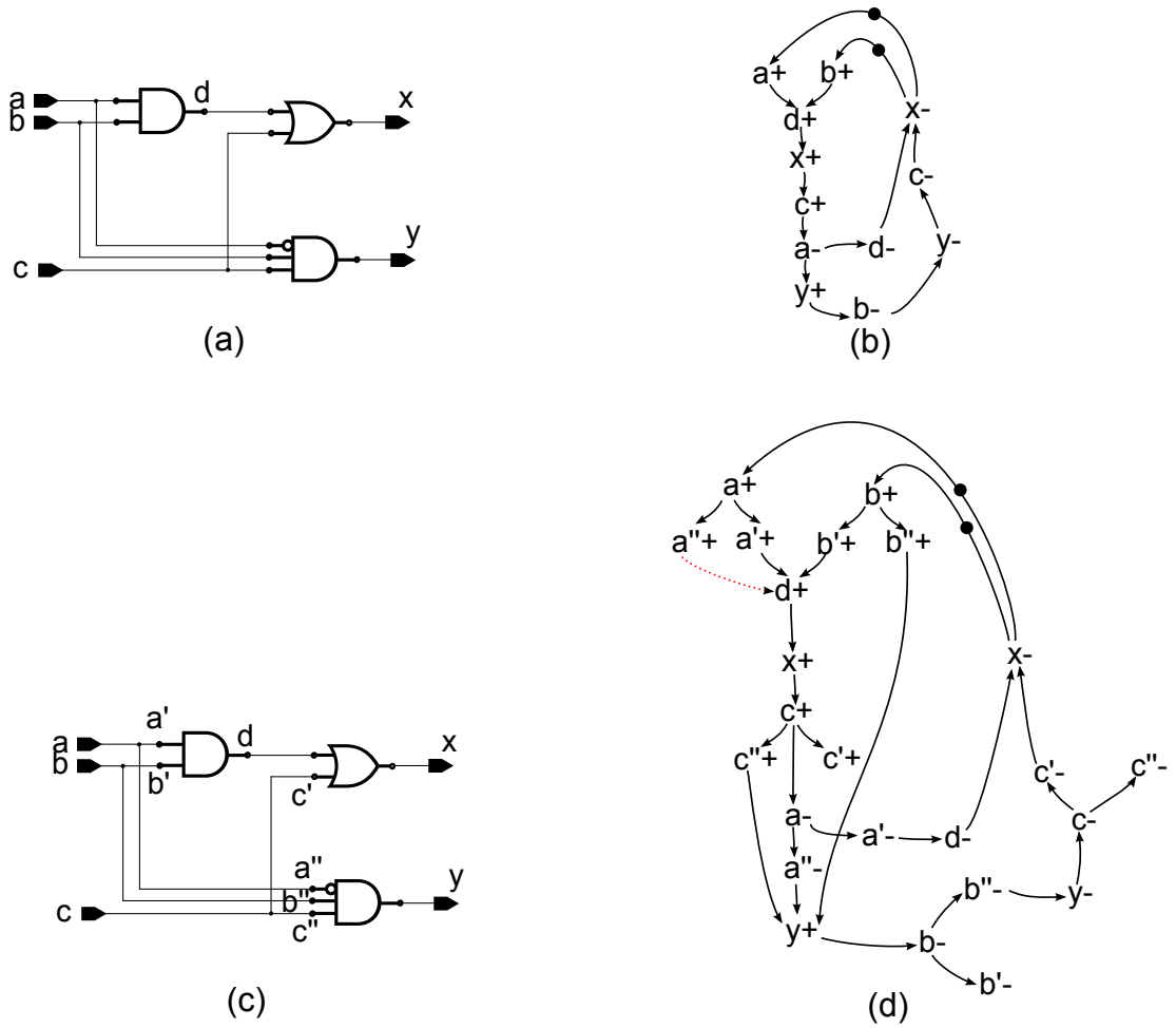
Figure 4.4: (a) An SI circuit, (b) the STG corresponding to (a), (c) The SI circuit with all wires explicitly denoted by signals and (d) the STG corresponding to (c) when the isochronic fork assumption is removed -
