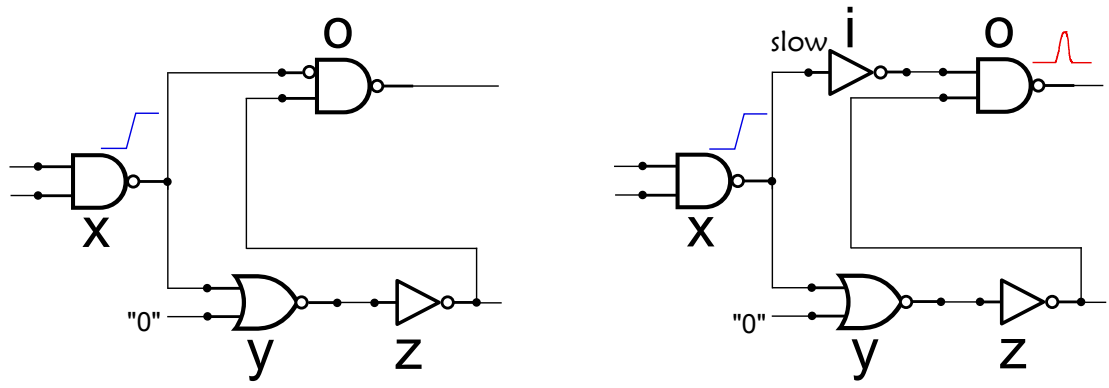
Figure 4.1: Glitches caused by inverter delay -
