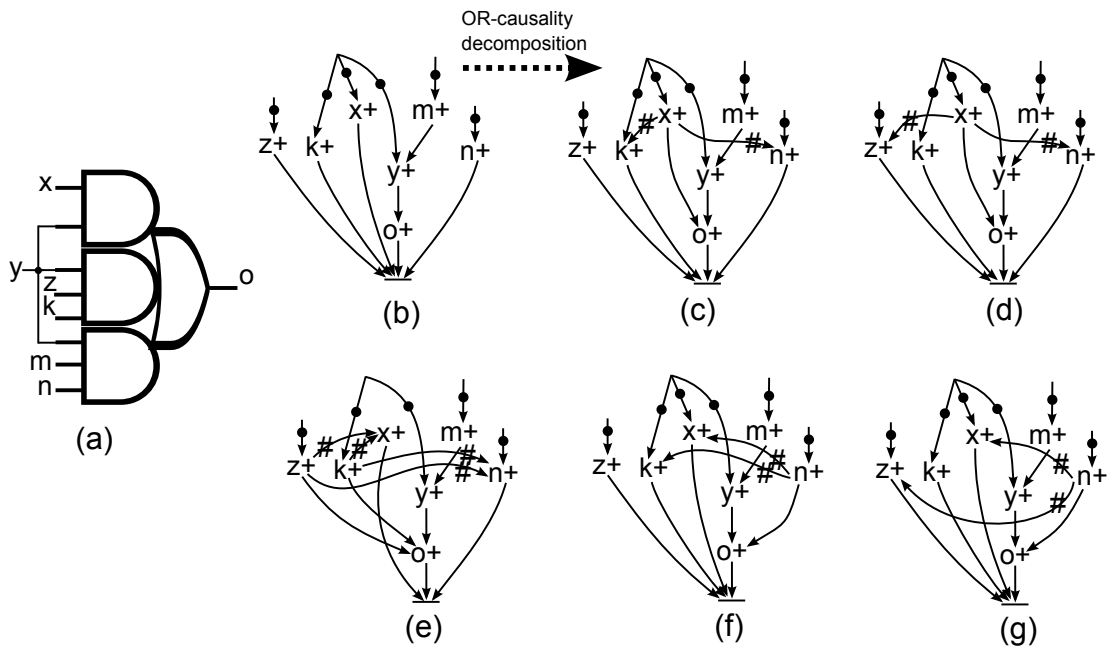
Figure 6.5: OR-causality decomposition example. (a) the gate, (b) STG segment before decomposition and (c)-(g) resulting subSTG segments -
