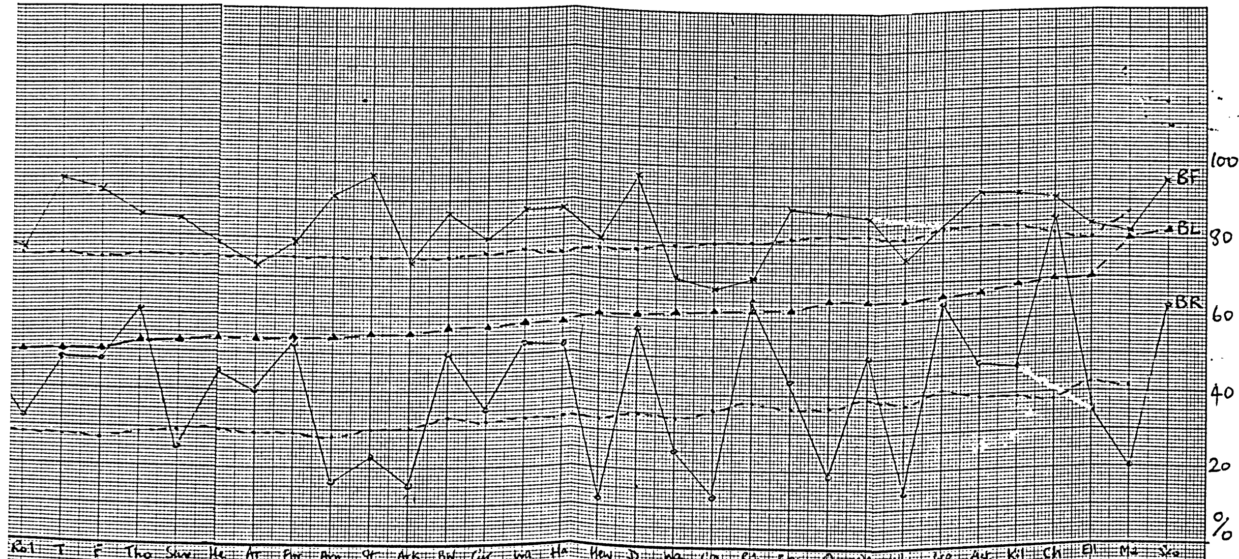
Figure B53: Boosted F_s , % F_s ; boosted L_s , % L_s ; boosted R_s , % R_s ; dependent, for Gps I, II, III, ranked on BL, and showing the BL/BF (top) and BL/BR (bottom) cumulative mean differences.
